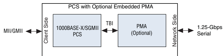
Figure 1-4. 1000BASE-X/SGMII PCS with Optional PMA
