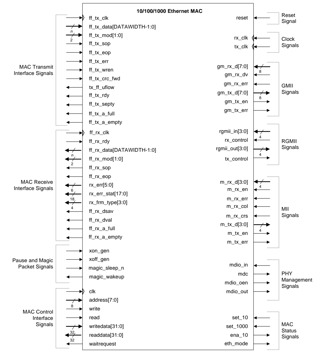
Figure 7–1. 10/100/1000 Ethernet MAC Signals
