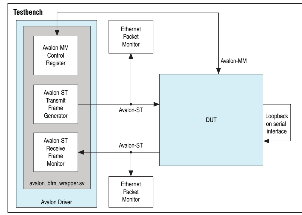
Figure 5-3. Testbench Block Diagram
